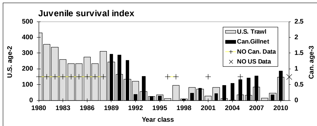
Fig. 2. Juvenile survival index of fish stocked into U.S. and Canadian waters. The index is the CUE of juvenile fish corrected for the number originally stocked. In U.S. waters the index is the overall catch of 2-year old fish per 500,000 yearlings stocked a year earlier; in Canadian waters the index is the CUE (per standard gillnet) of 3-year old fish per 500,000 yearlings stocked two years earlier.
