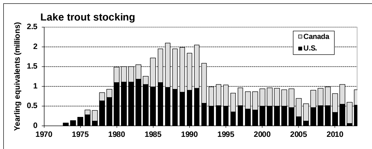
Fig. 1. Numbers of Lake Trout stocked in U.S. and Canadian waters expressed as spring yearling equivalents (1 fall fingerling = 0.41 spring yearling; Elrod et al. 1995).
