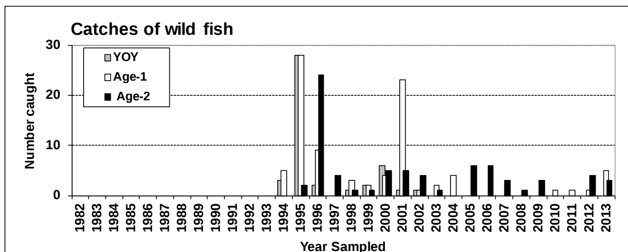
Fig. 5. Numbers of wild fish caught annually in U.S. bottom trawling (four total) and gillnetting (one total) surveys. Wild juveniles (age 0-2) can be distinguished from hatchery fish by size, color, shape, and lack of tag or fin clip.
