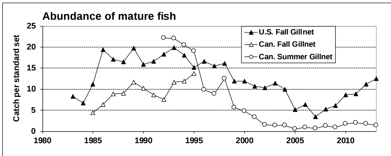
Fig. 3. Abundance of mature fish in U.S. and Canadian waters, measured as catch per standard gillnet. Fall gillnet Lake Trout surveys have been conducted in the U.S. and Canadian waters since the early 1980s; in Canadian waters the fall surveys were discontinued in 1995 and Lake Trout are now assessed in summer fish community gillnet surveys.
