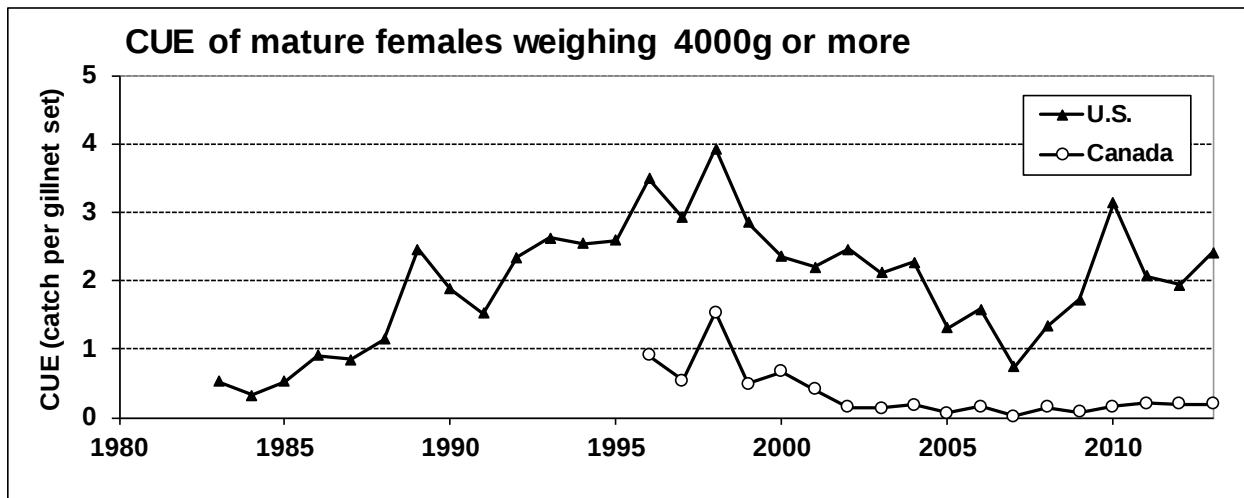
Fig. 4. Abundance index of mature female Lake Trout \geq 4000g , from September U.S. adult Lake Trout gillnetting assessment and summer Canadian fish community index gillnetting.
